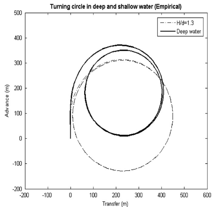
Fig. 13. Comparison of simulated turning trajectories in deep and shallow water based on empirical equations.
