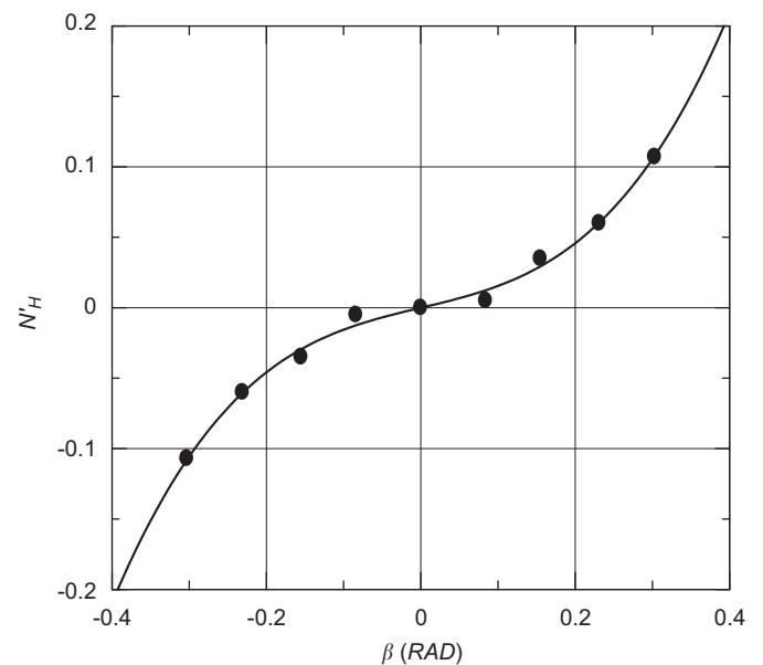
Fig. 5. Yaw moment (pure sway- shallow water).
