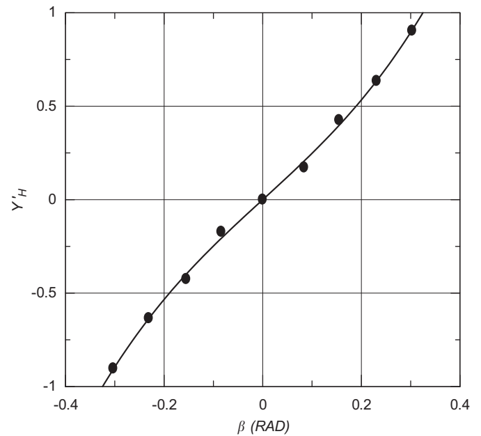
Fig. 4. Sway force (pure sway-shallow water).
