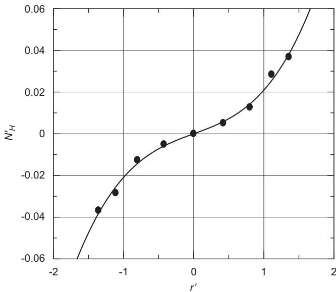
Fig. 7. Yaw moment (pure yaw-deep water).
