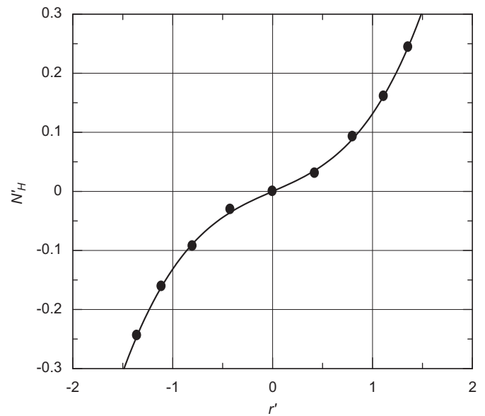
Fig. 9. Yaw moment (pure yaw-shallow water).
