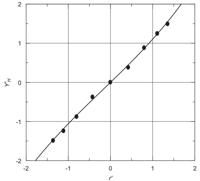
Fig. 8. Sway force (pure yaw-shallow water).
