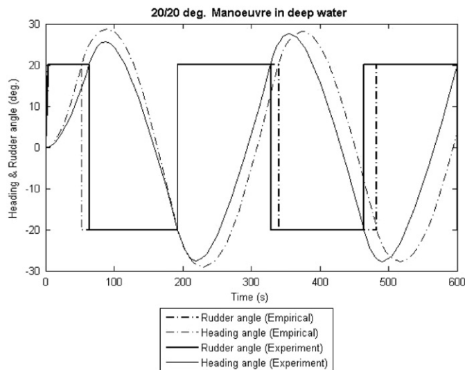
Fig. 12. Comparison of time histories of 20°/20 zig-zag [speed = 7 Knots].
